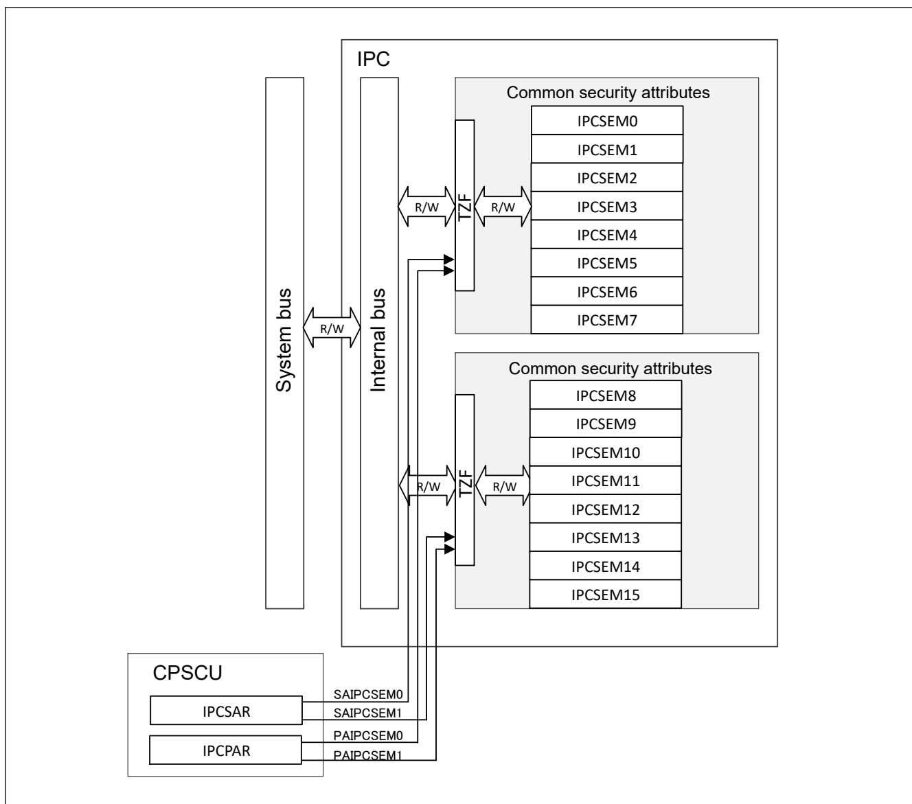
Figure 3.2 IPCSEM register
